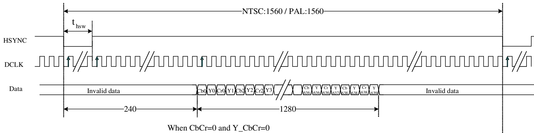
Fig.8 YUV640 Input Horizontal Timing Chart
