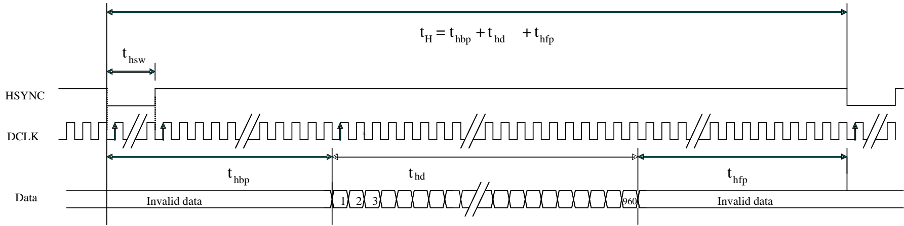
Fig.1 UPS051 Input Horizontal Timing Chart
