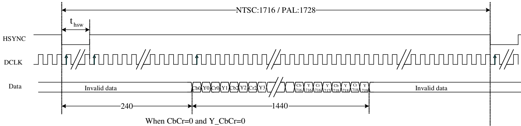
Fig.7 YUV720 Input Horizontal Timing Chart
